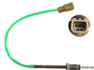
SENSOR EXHAUST GAS TEMPERATURE RENAULT TRAFIC 14>
